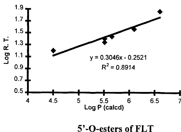
Figure 1. The correlation between Log retention time and lipophilicity (Log P) for 5'-O-esters of FLT.
